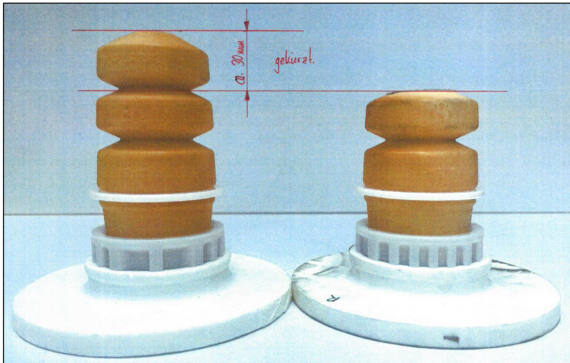
links: original Anschlagpuffer incl. Federteller rechts: ca. 30 mm gekürzter original Anschlagpuffer incl. Federteller left: OE bump stop with spring plate right: approx. 30 mm shortened OE bump stop with spring plate
